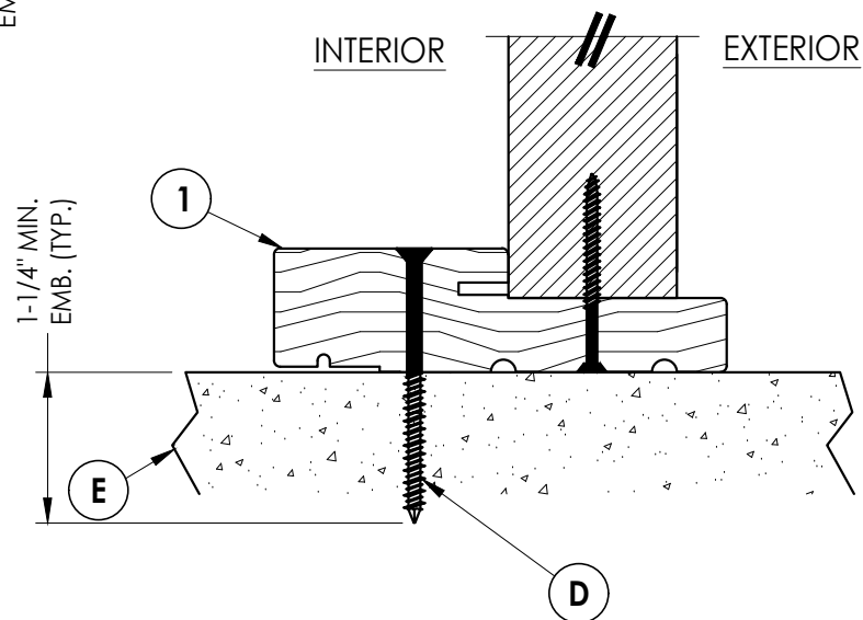
5 3 VERTICAL CROSS SECTION Outswing Sill
