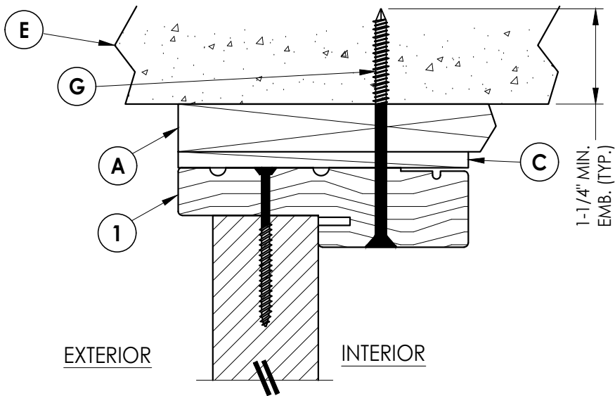
2 3 VERTICAL CROSS SECTION Outswing 1X Buck Construction
