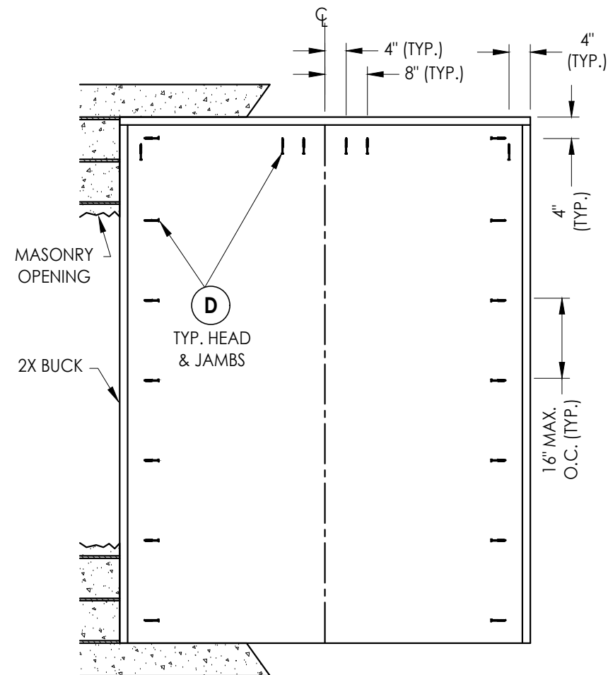
BUCK ANCHORING XX
