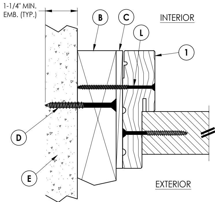
4 HORIZONTAL CROSS SECTION 2 Outswing 1X Buck Construction
