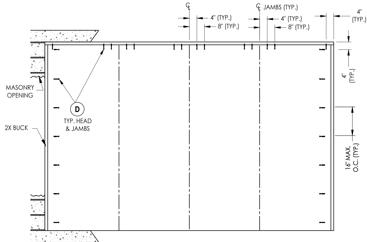
BUCK ANCHORING OXXO
