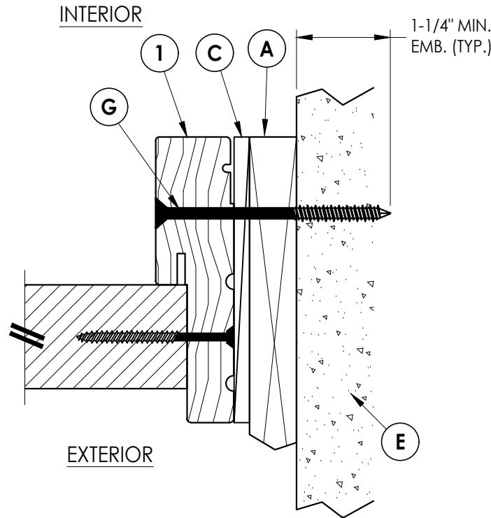
3 HORIZONTAL CROSS SECTION 2 Outswing 1X Buck Construction
