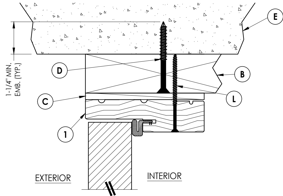
1 3 VERTICAL CROSS SECTION Outswing 2X Buck Construction
